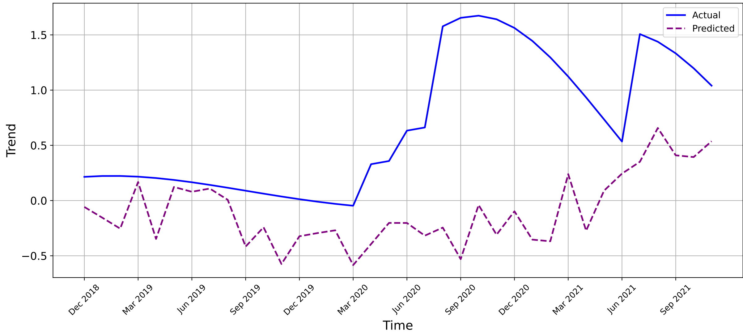
Solution_HYPERGAME_Mentions - Validation
